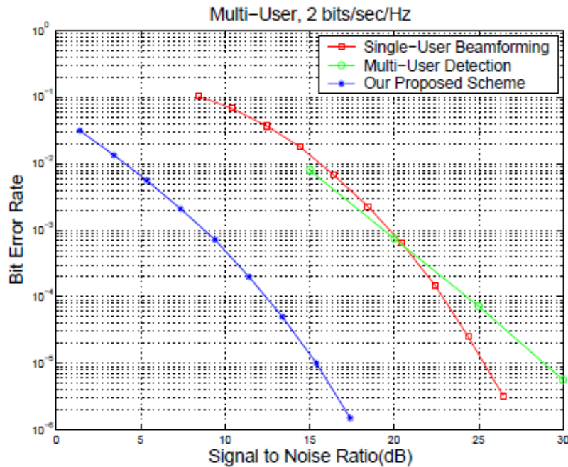
Figure 2: Simulation results for 2 users each with 4 transmit antennas and 2 receivers each with 4 receive antennas. The constellation is QPSK.
